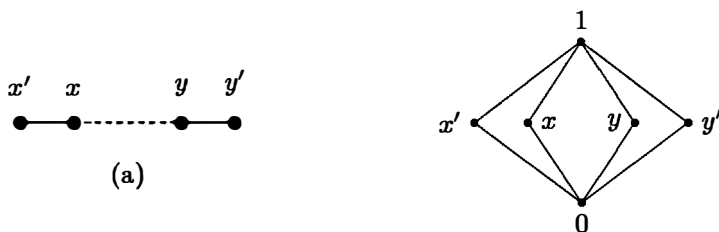
Figure 4. Greechie diagram for the lattice MO2 and its Hasse diagram. The dashed line indicates that the unconnected blocks belong to the same Greechie diagram.
