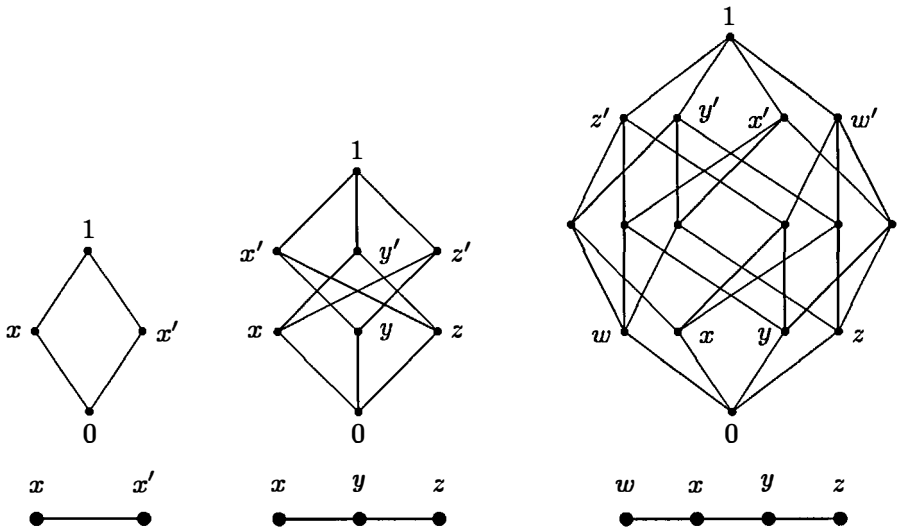
Figure 2. Greechie diagrams for Boolean lattices 2^2 , 2^3 , and 2^4 , labelled with the atoms of their corresponding Hasse diagrams shown above them. ( 2^4 was adapted from [Beran, 1985, Fig. 18, p. 84].)
