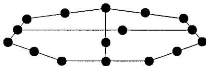
Figure 11. An OML that is nOA for n = 3, 4, 5, 6 but which is neither nGO for any n nor MGO.
