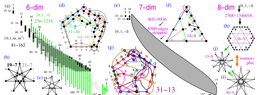
Figure 3. (a) Distributions of six-dim critical non-KS NBMMPHs obtained from two different submasters—see text; (b) the smallest critical non-KS NBMMPH obtained from the former class by M3 , which has a parity proof; (c) an even smaller critical non-KS NBMMPH obtained from it by hand, which has a parity proof; (d) the smallest critical non-KS NBMMPH obtained from the latter class by M1 ; (e) distributions of seven-dim critical non-KS NBMMPHs—see text; (f) 14-8 non-KS NBMMPH, one of the smallest non-KS NBMMPHs obtained via M3 from the smallest KS NBMMPH, 34-14; (g) 31-13 also obtained from the 34-14 (no m = 1 vertices essential for criticality); (h,i) isomorphic eight-dim KS MMPHs with the smallest number of hyperedges (9) used to generate the 15-9 non-KS NBMMPH in (j); (h–j) MMPHs with parity proofs; strings and coordinatizations are given in Appendix A.
